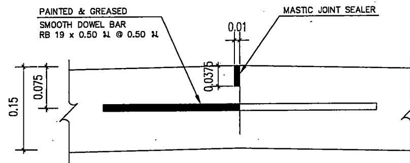
( CONSTRUCTION JOINT )
